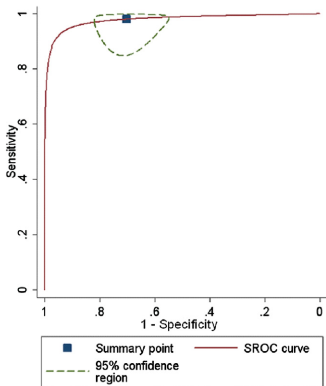
Figure 6. Summary receiver operating characteristic plot. The figure shows the summary curve, along with the point estimate and the 95% confidence region.
